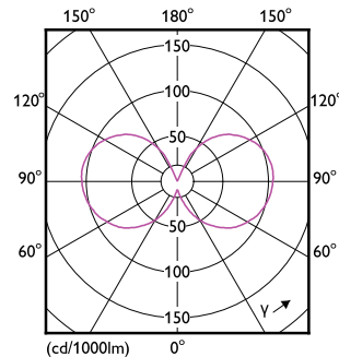
Light Distribution Diagram - CorePro LEDLusterND6.5-60W P45 E27827CLG
