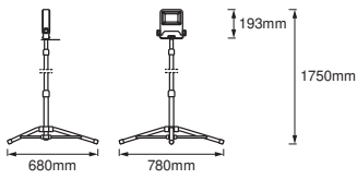
LED WOKRLIGHT 1x30W TRIPOD
