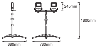
LED WOKRLIGHT 2x50W TRIPOD
