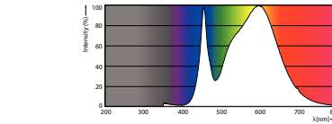
Spectral Power Distribution Colour - TForce Core LED HPL 36W E27 840 FR
